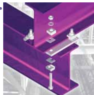
Beam Clamp® A KEE SAFETY PRODUCT
